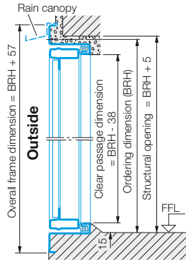
Single leaf door with stepped floor
