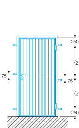
Position of anchors
