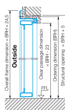
Single leaf door (supplied without bottom threshold)
