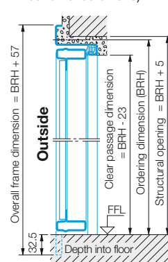
Single leaf door (supplied with bottom threshold as standard, will be removed on site)
