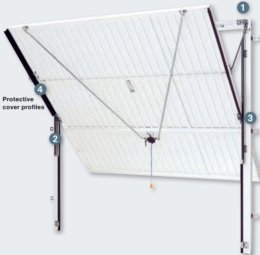
1 Cable drum
