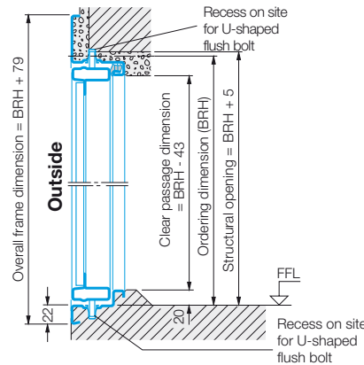
Door with flat floor
