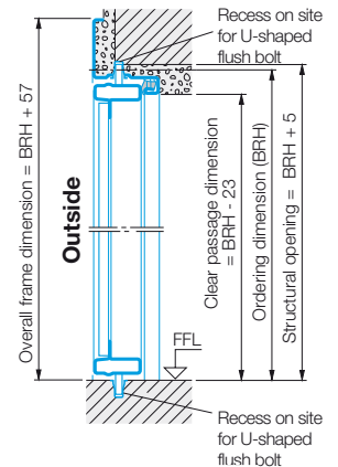
Door with stepped floor
